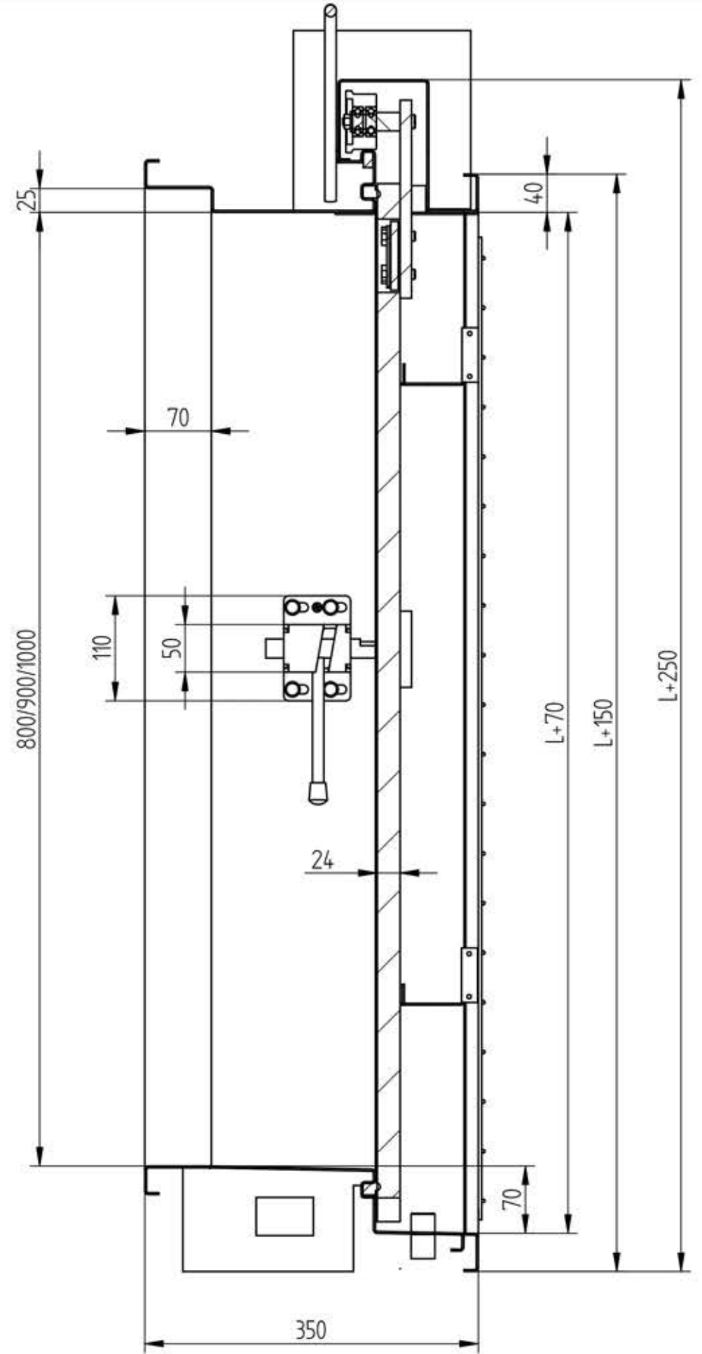
SECTION B-B
